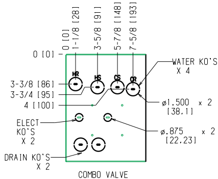
COMBO VALVE
