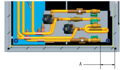
4 PIPE HEATING/COOLING
